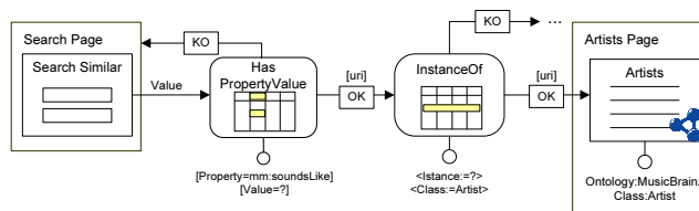
Figure 1: A piece of WebML model describing a Semantic Web application.
