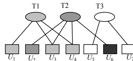
Figure 2. Similar Annotations
