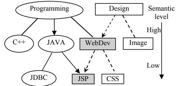
Figure 4. Hierarchical structure
