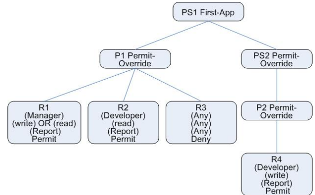
Figure 1: Example Policy
